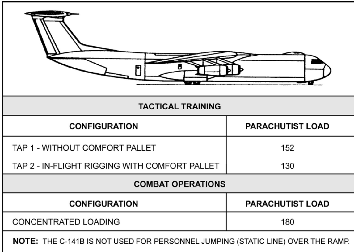
Figure 16-8. C-141B Starlifter.
