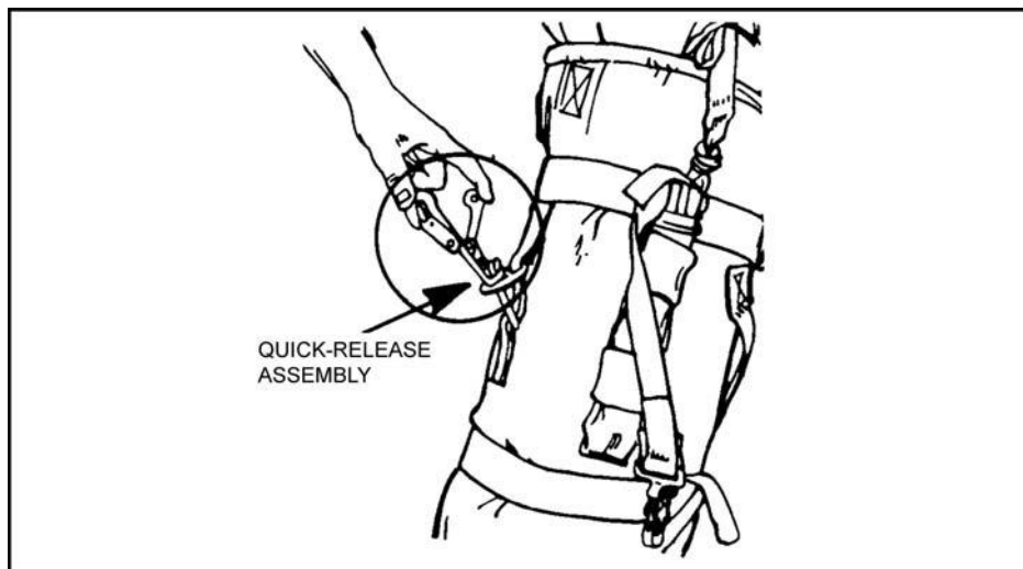
Figure 12-37. Quick-release assembly.
